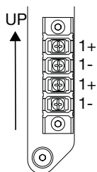
Screw terminal input/link wiring
