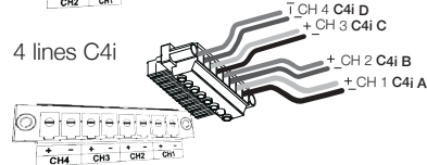
Euroblock 4/8-p amplifier output wiring
